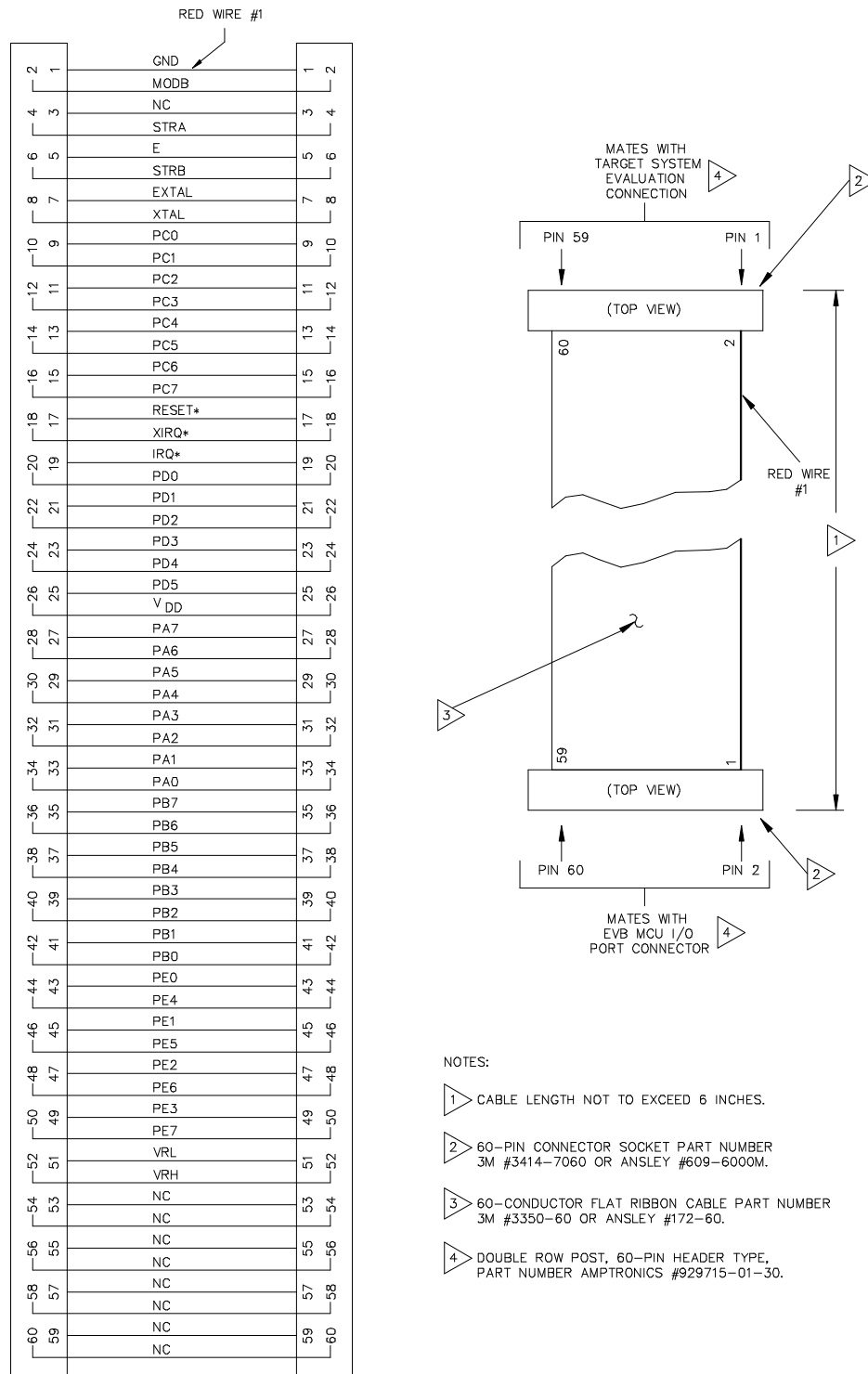
Figure 2-3. MCU I/O Port Extension Cable Assembly Diagram
