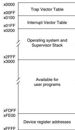
Figure A.1 Memory map of the LC-3
