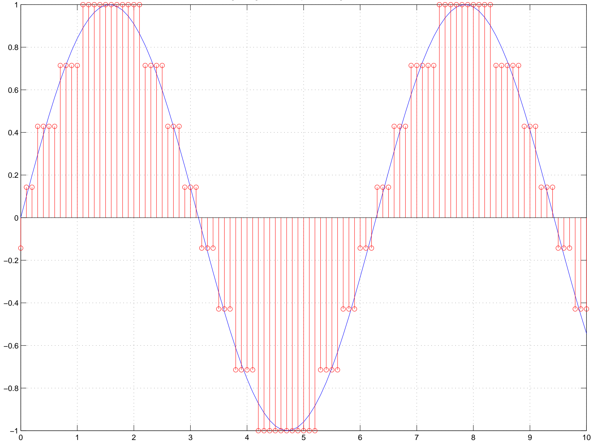
original signal and the quantized signal for N = 8
