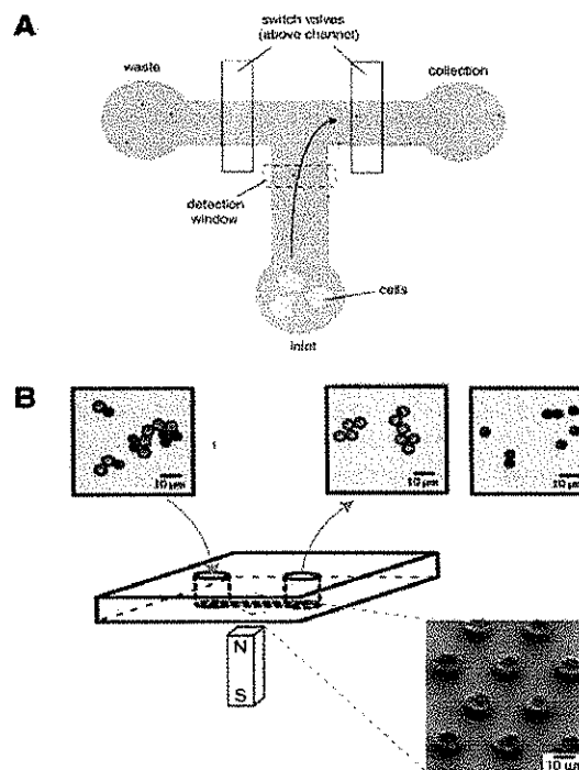
Figure 4. Miniaturized sorting devices. (A) Microfabricated fluorescence-activated cell sorter. Samples containing fluorescently labeled molecules flow from the input well to the detection window. Detection of fluorescence triggers pneumatically actuated switch valves that force the cells to flow to the collection well [62]. (B) Magnetic filtration device. Next to a permanent magnet, the nickel posts create a large local magnetic field gradient and capture 4.5 \mu\text{m} superparamagnetic beads (colored) from a mixture also containing nonmagnetic beads (not colored). Figure adapted from [64].
