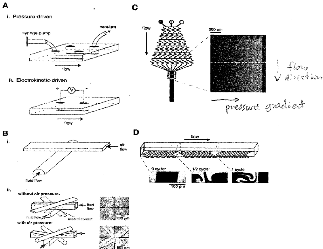
Figure 1. Toolbox for PDMS-based microfluidic bioassays. (A) Methods for driving fluid flow. (i) Pressure-driven flow using a vacuum at the outlet or a syringe pump at the inlet. (ii) Electrokinetic flow using a voltage applied across the microchannel. (B) Switches and valves for control of fluid movement. (i) Pneumatically actuated monolithic valve. When pressure is applied above, flow in the bottom rounded channel stops [18]. (ii) Channel crossing in which the fluid flow can be switched. When air pressure is applied above and below the crossing, the fluid turns 90° instead of flowing straight. Figure adapted from [20]. (C) Gradient generator using laminar flow. A solution or surface-bound molecular gradient is generated perpendicular to the direction of fluid flow in the microchannel. Figure adapted from [31]. (D) Chaotic mixer. Neighboring streams of fluids are passively mixed. Homogeneity is observed after 16 cycles of the staggered herringbone structure. Figure adapted from [32].
