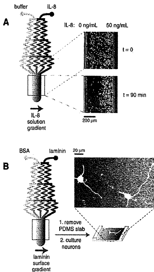
Figure 5. Studying the responses of cells to molecular gradients in microchannels. (A) Study of chemotaxis of neutrophils in a solution gradient of IL-8. In a linear gradient of IL-8 from 0 ng/mL to 50 ng/mL, neutrophils migrated to the region of highest IL-8. Figure adapted from [72]. (B) Dependence of axonal specification of hippocampal neurons on surface-bound gradients of laminin. A surface-bound gradient of laminin is formed from a solution gradient. Neurons cultured on the gradients exhibit preferential axonal specification in the direction of increasing laminin concentration. Figure adapted from [73].
