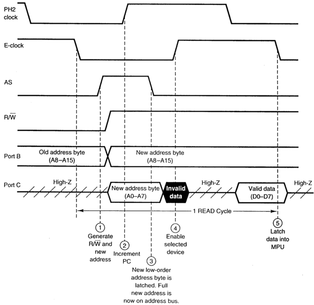
FIGURE 5.6 68HC11 MPU bus activity during a READ cycle in the expanded mode.
