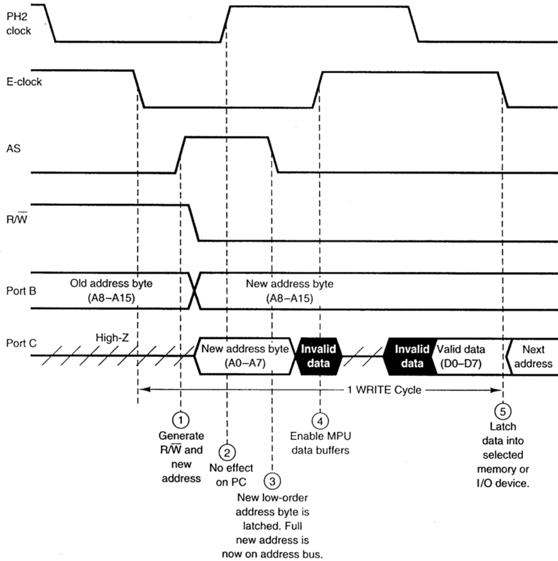
FIGURE 5.7 68HC11 MPU bus activity during a WRITE cycle in the expanded mode.
