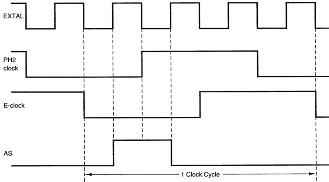
FIGURE 5.5 Timing relationships for the 68HC11 MPU clocks and AS signal in the expanded mode.
