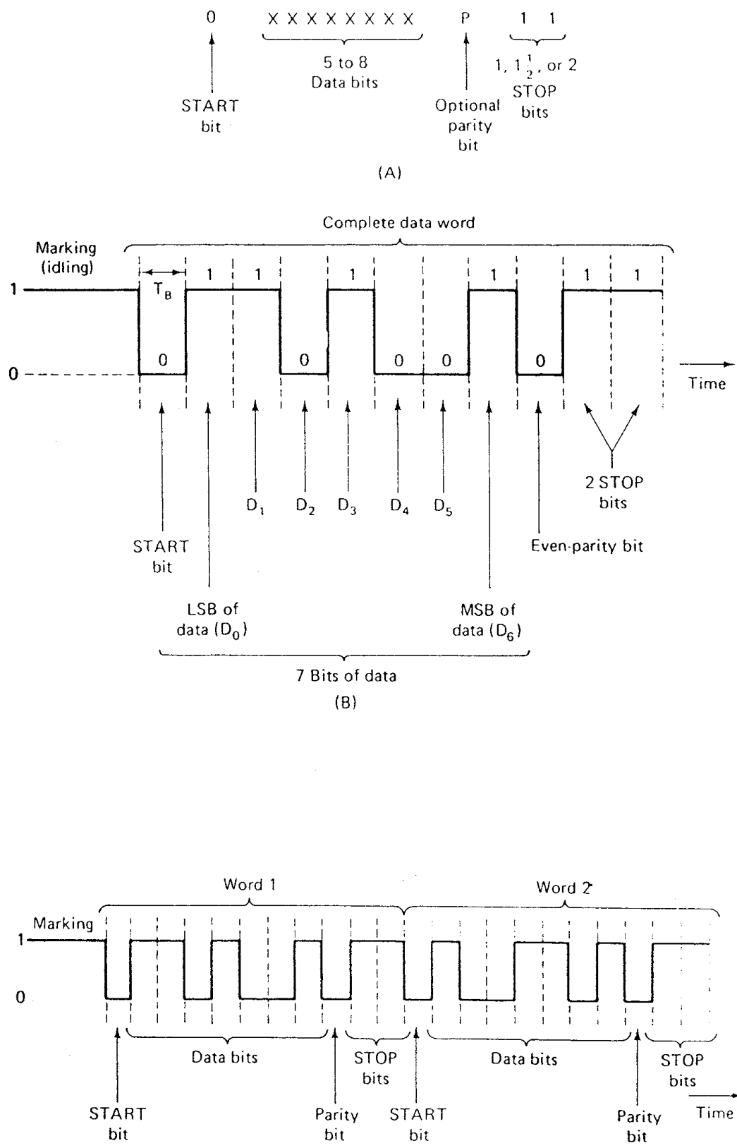
FIGURE 9.8 Transmitted serial signal for two consecutive words.
