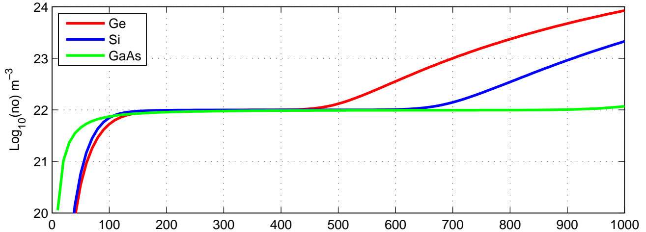
Absolute Carrier Concentration ( N_D = 10^{22} \text{ m}^{-3} )
