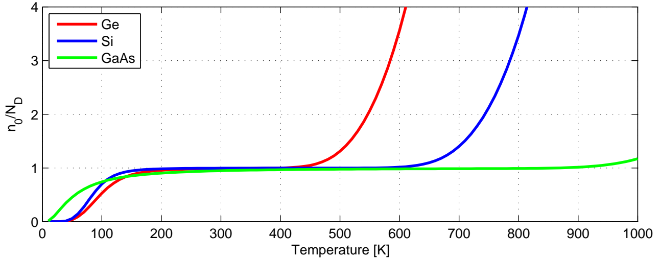
Relative Carrier Concentration n_0/N_D ( N_D = 10^{22} \text{ m}^{-3} )
