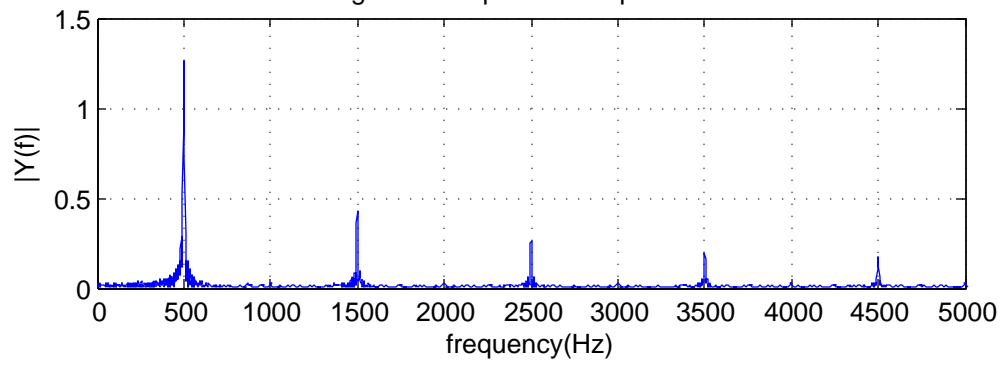
Magnitude response of Square wave
