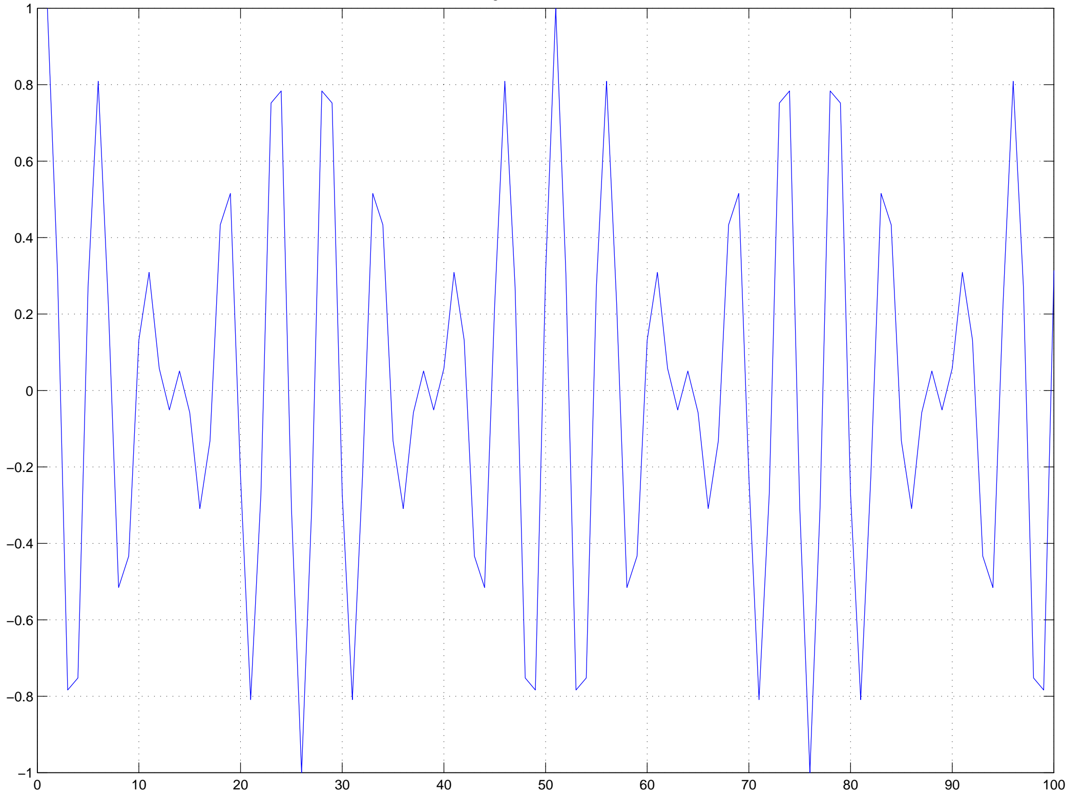
DSBSC signal fin1=1KHz fin2=10KHz
