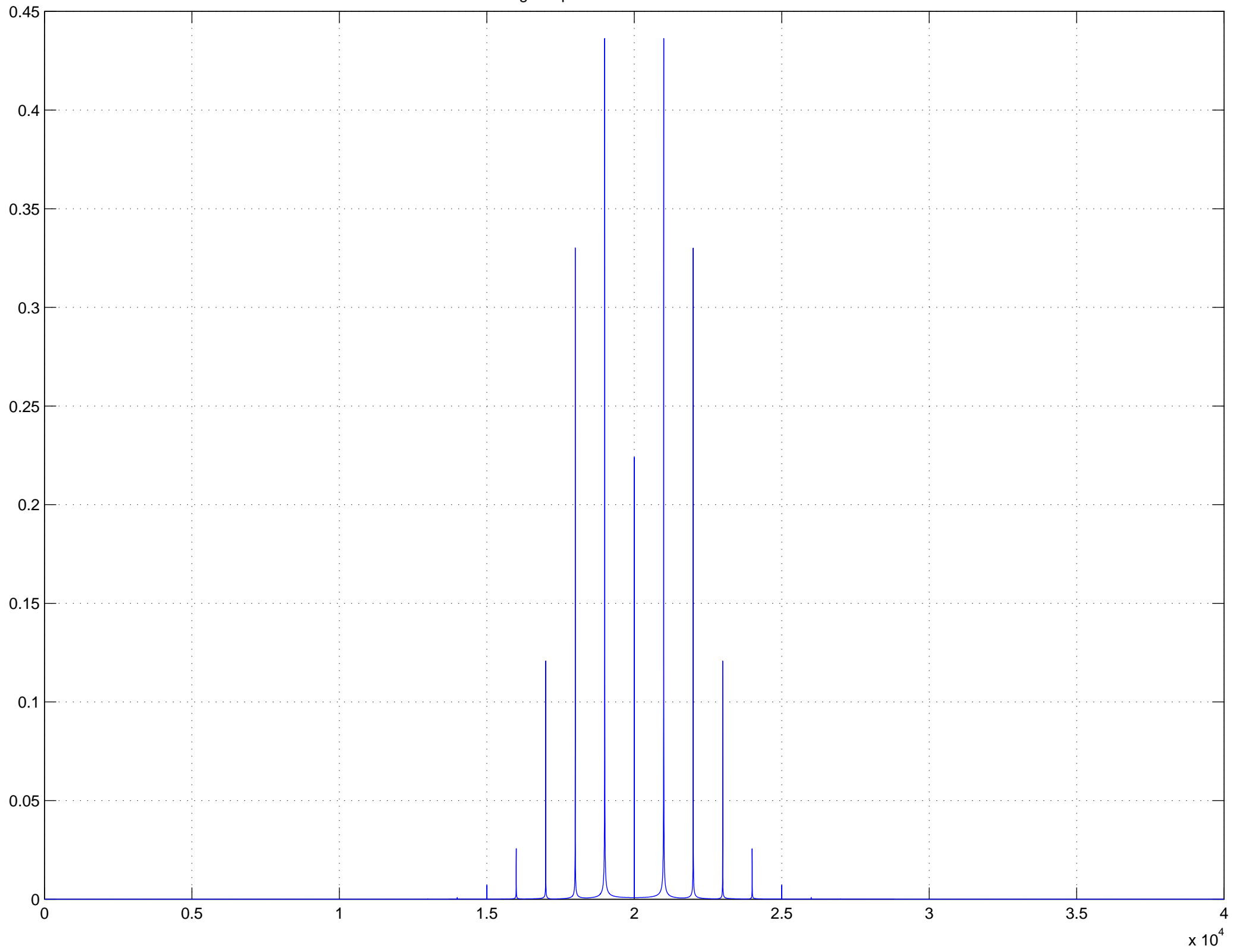
FM signal spectrum for beta=2 and f2=1000
