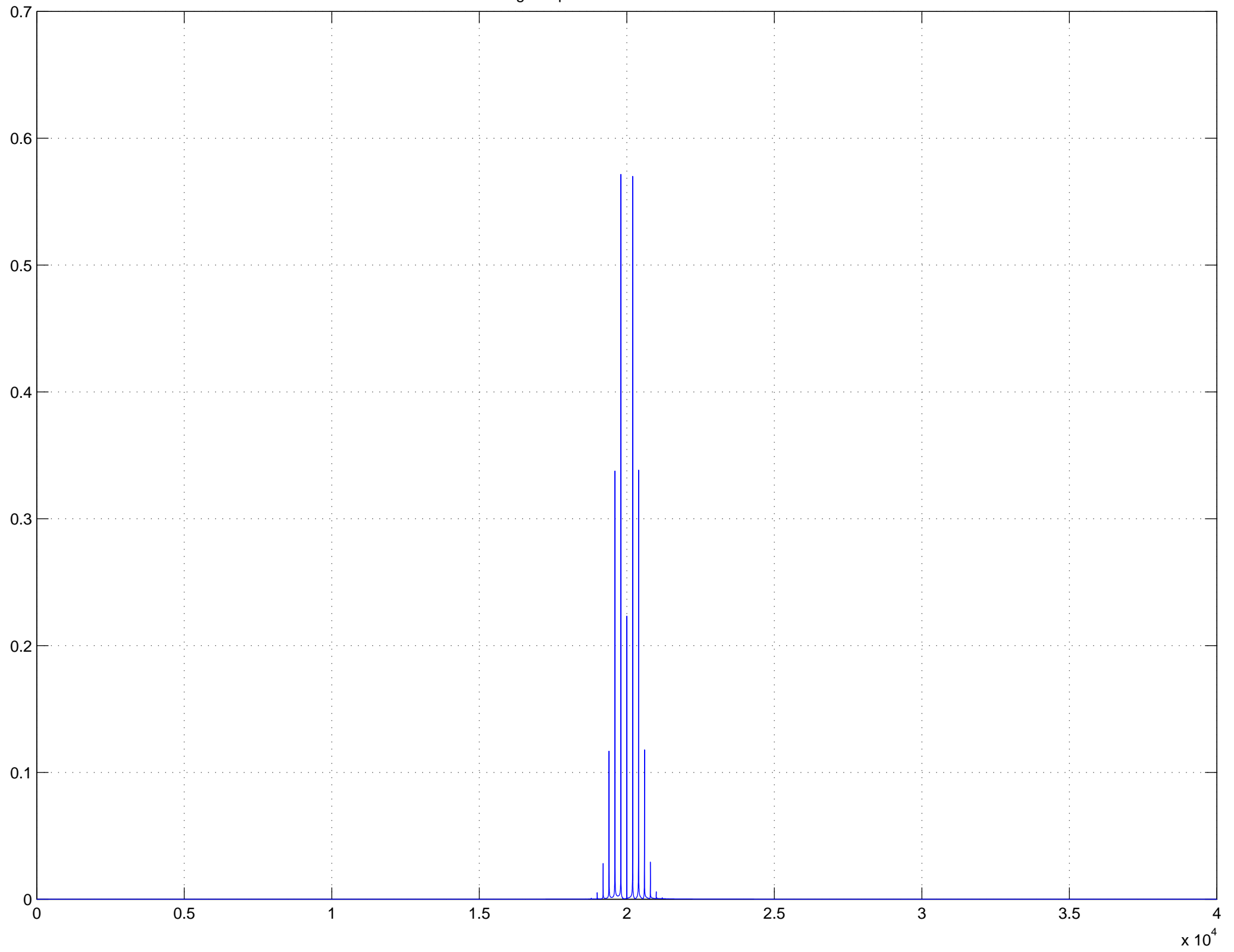
FM signal spectrum for beta=2 and f2=200
