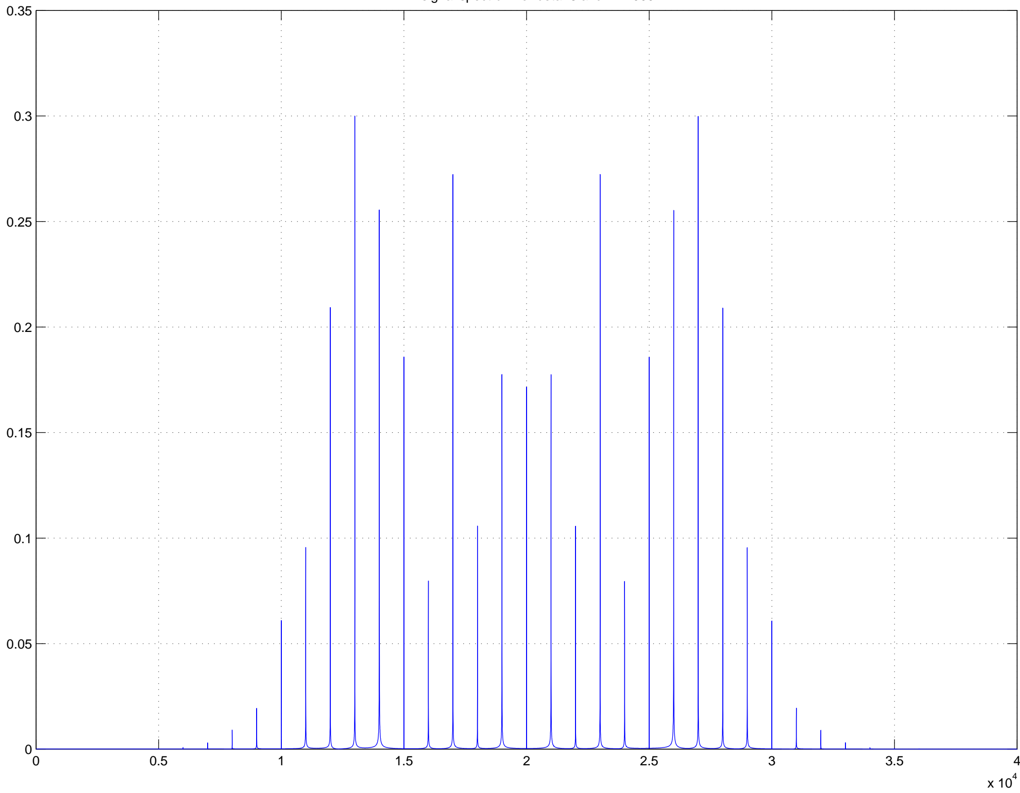
FM signal spectrum for beta=8 and f2=1000
