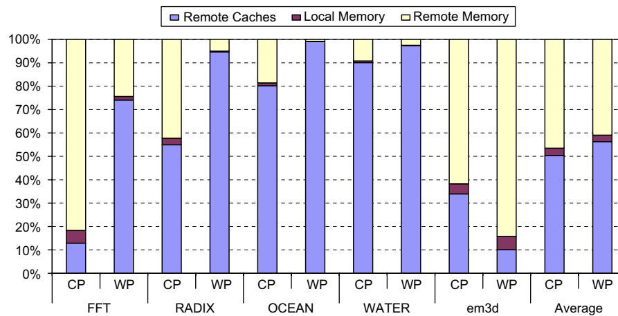
Fig. 9. Servicing coherence transactions for directory-based SMPs for the correct path (CP) and the wrong-path (WP).
