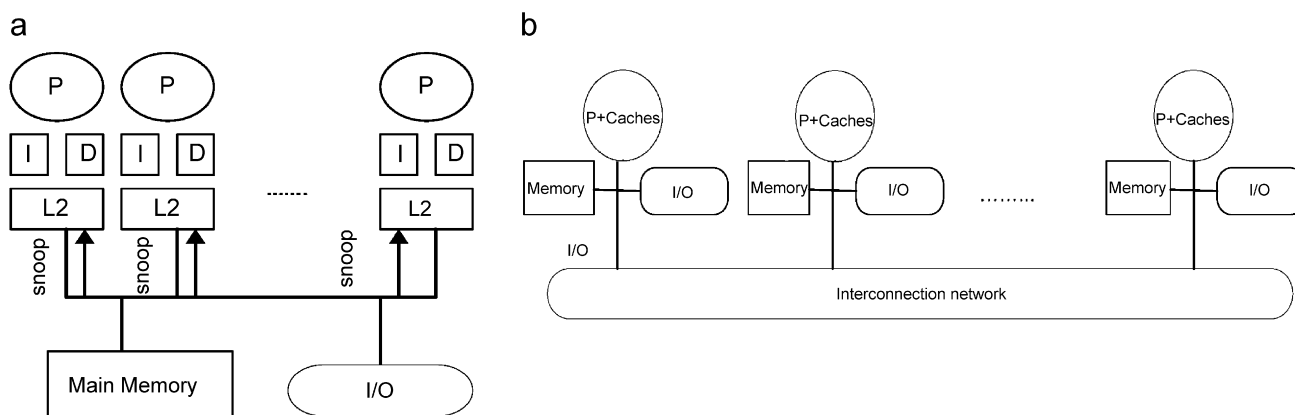
Fig. 2. (a) Broadcast and (b) directory based SMPs.
