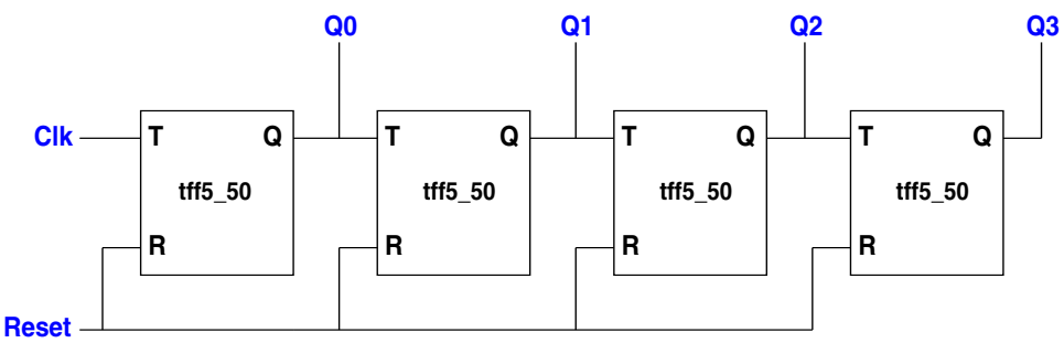
Schematic for Dynamic Asynchronous Counter
