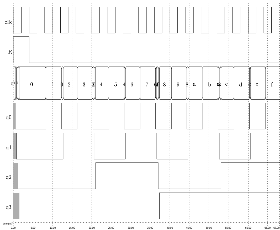
Irsim plot created from ascntr1_50
