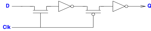
Schematic for Dynamic D Flip-Flop
