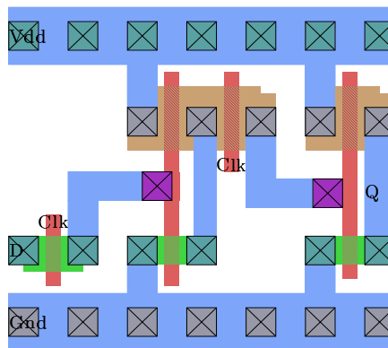
Magic plot for dff2_50
