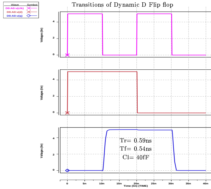
Hspice file created from dff2_50
