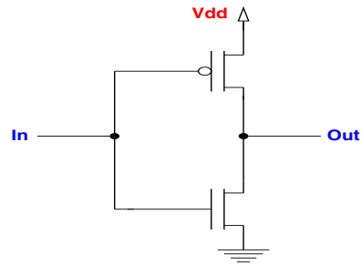
Schematic for Inverter
