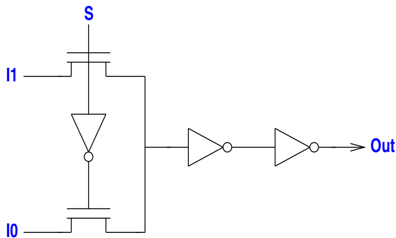
Schematic for mux2to1_50
