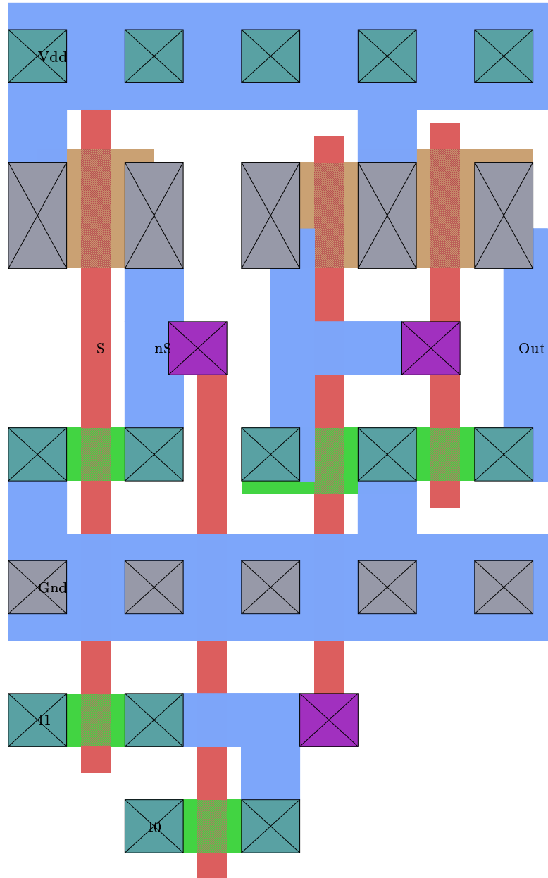
Magic plot for mux2to1_50
