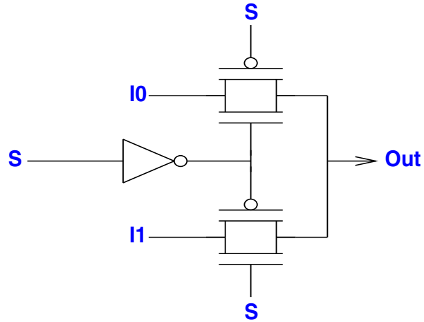
Schematic for mux2to1c_50
