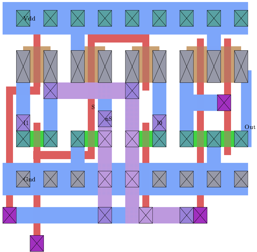
Magic plot for mux2to1c.50
