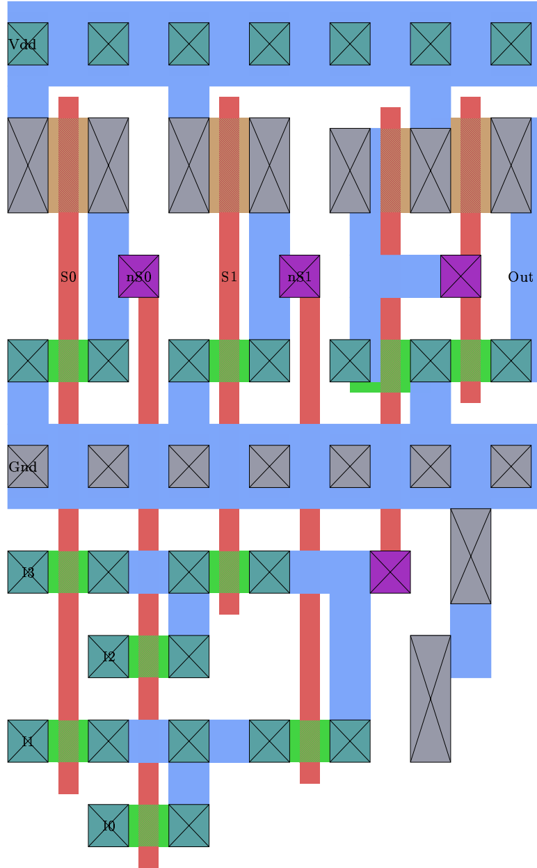
Magic plot for mux4to1_50
