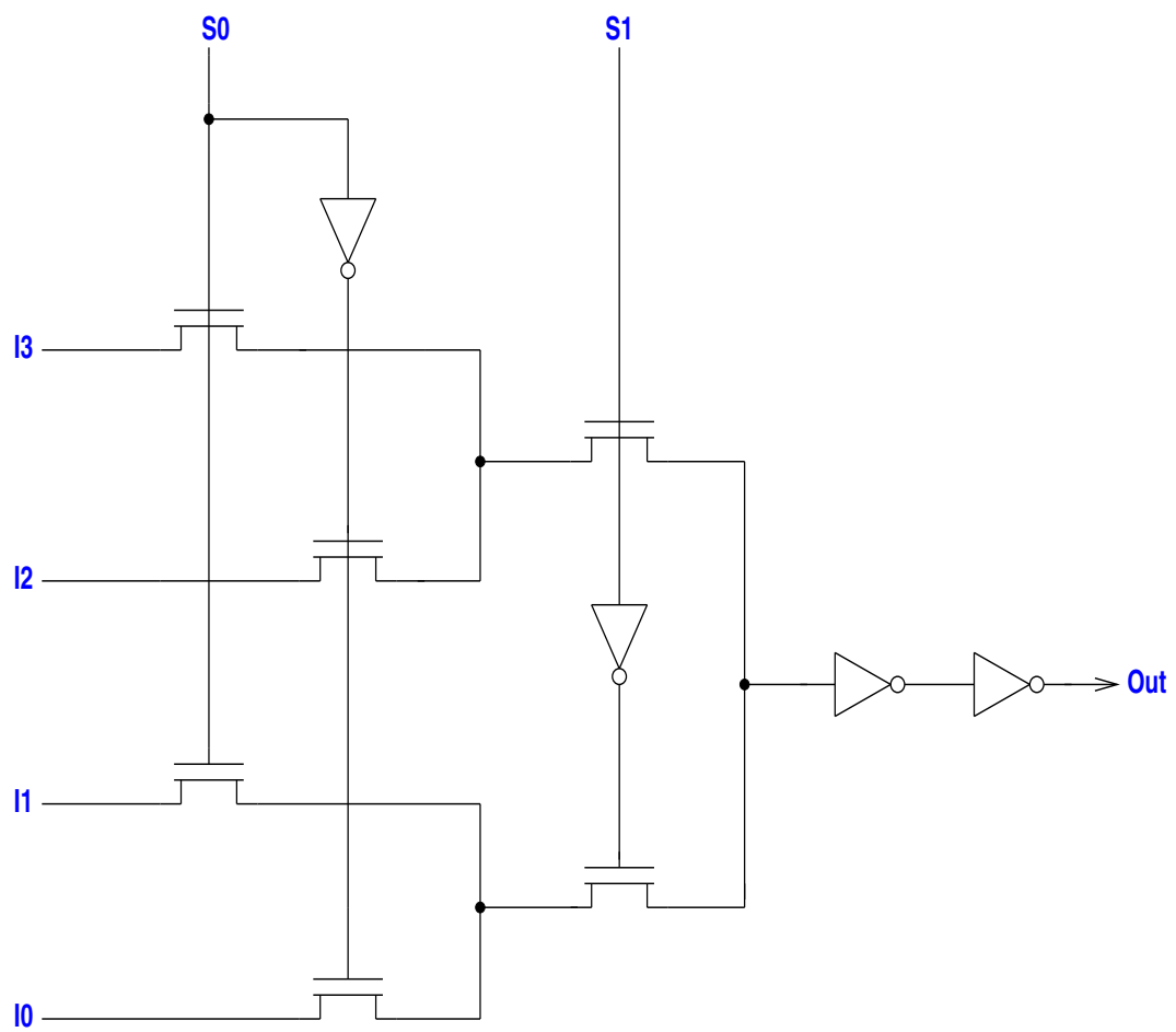
Schematic for mux4to1_50
