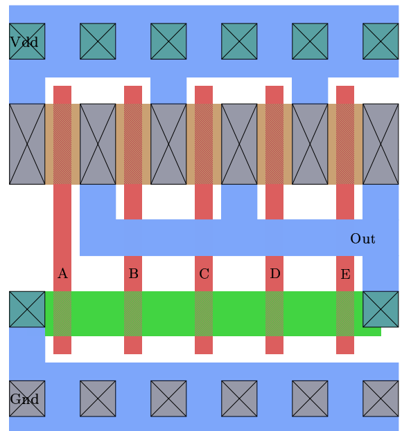
Magic plots for nand4_50 and nand5_50
