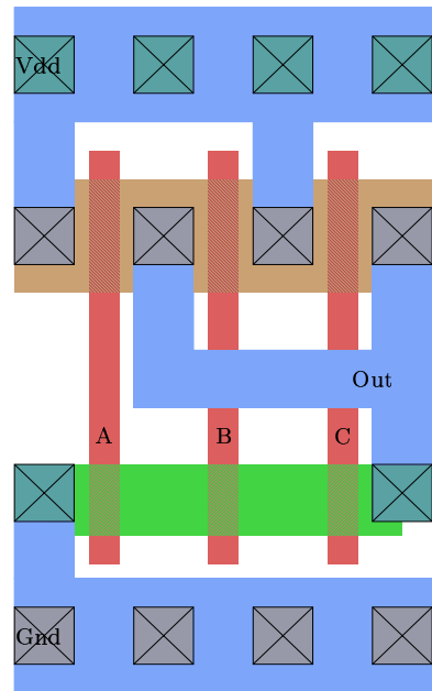
Magic plots for nand50 and nand3_50
