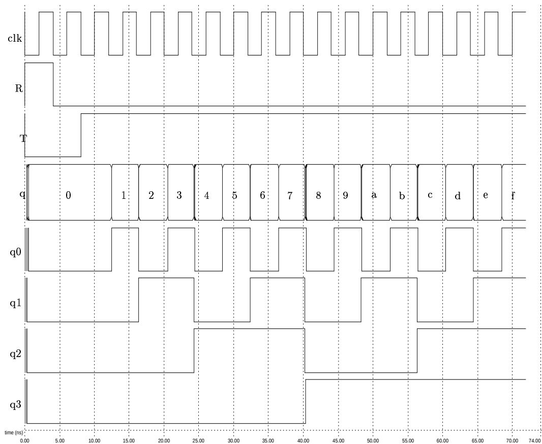
Irsim plot created from scntr1_50
