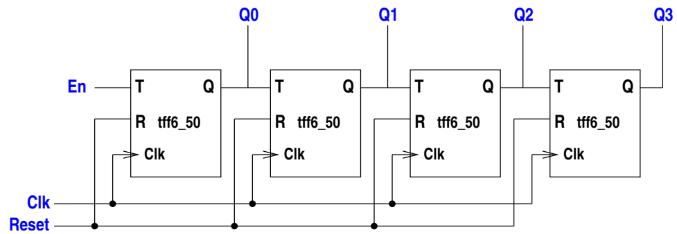
Schematic for Dynamic Synchronous Counter
