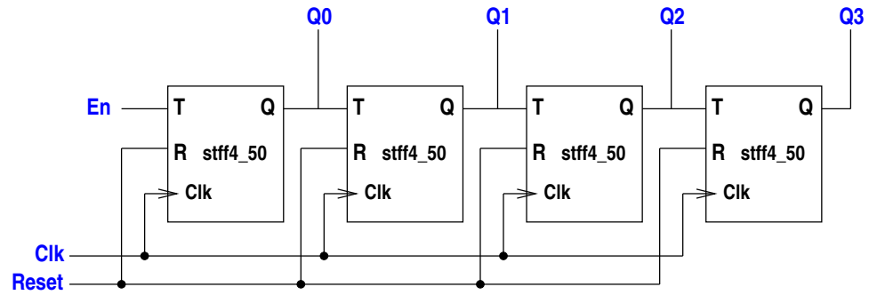
Schematic for Static Synchronous Counter
