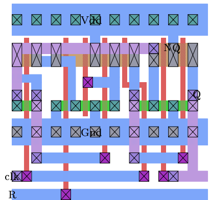
Magic plot for stff1_50
