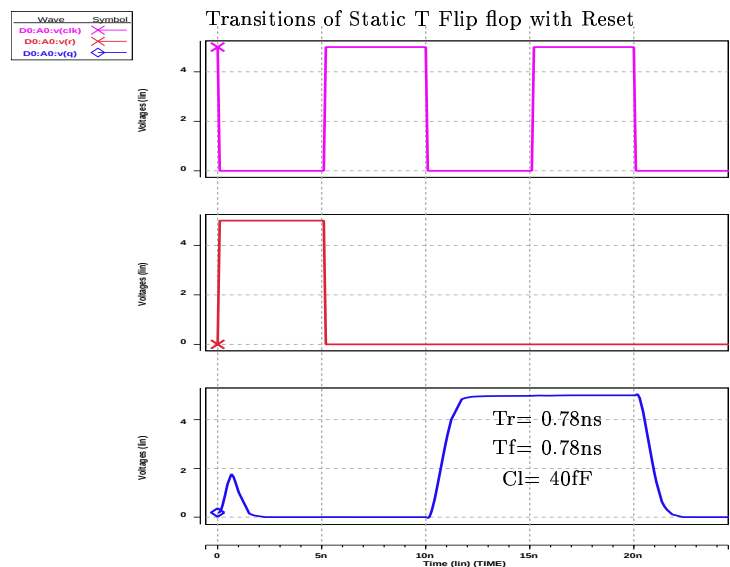
Hspice file created from stff1_50
