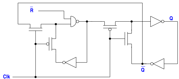
Schematic for Static T Flip-Flop with Reset
