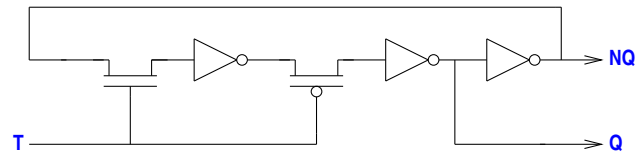
Schematic for Dynamic T Flip-Flop
