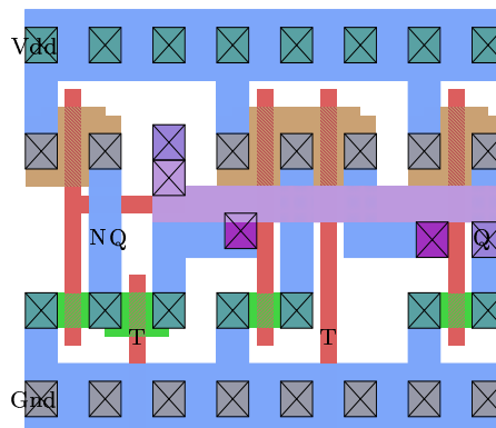
Magic plot for tff3_50
