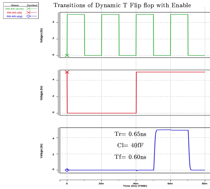
Hspice file created from tff4_50
