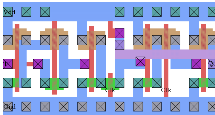
Magic plot for tff4_50
