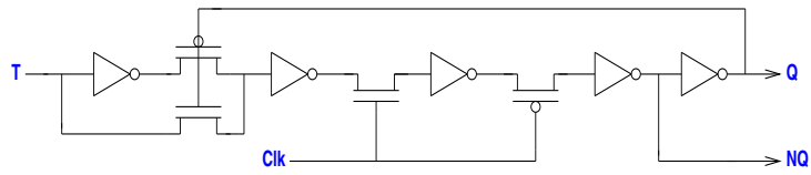
Schematic for Dynamic T Flip-Flop with Enable
