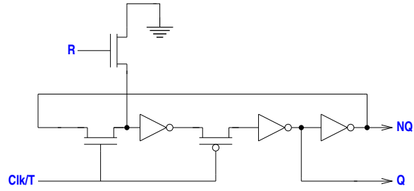
Schematic for Dynamic Flip-Flop with Reset
