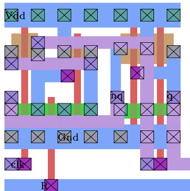
Magic plot for tff5_50
