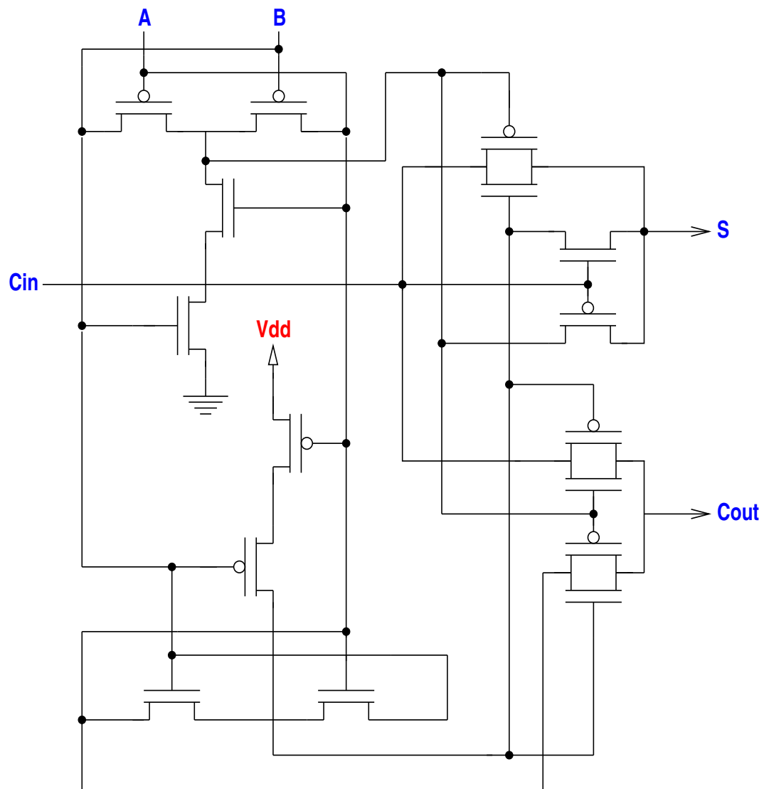
Schematic for Transmission Gate Full adder
