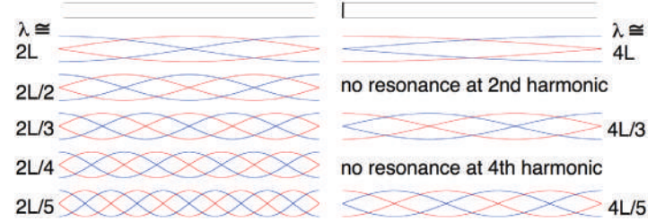
Figure 4. Resonant modes in cylindrical ducts of length L . Red, acoustic pressure; blue, acoustic flow. The open-open pipe (top left) has, at both ends, pressure nodes and flow antinodes. When one end is closed (top right), this boundary condition permits no acoustic flow and allows an antinode in pressure. The longest wavelength (lowest frequency) modes are at top. See www.phys.unsw.edu.au/jw/AT for more details.
