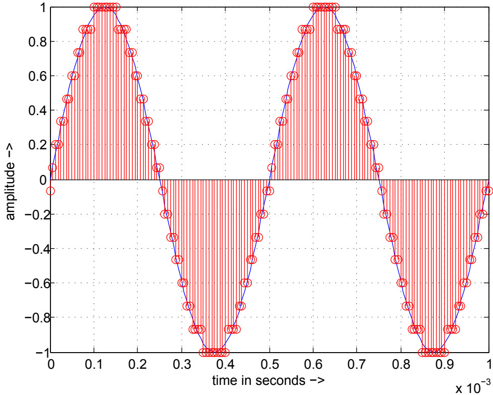
original signal and the quantized signal for N = 16
