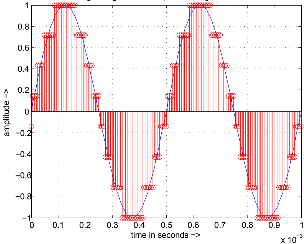
original signal and the quantized signal for N = 8
