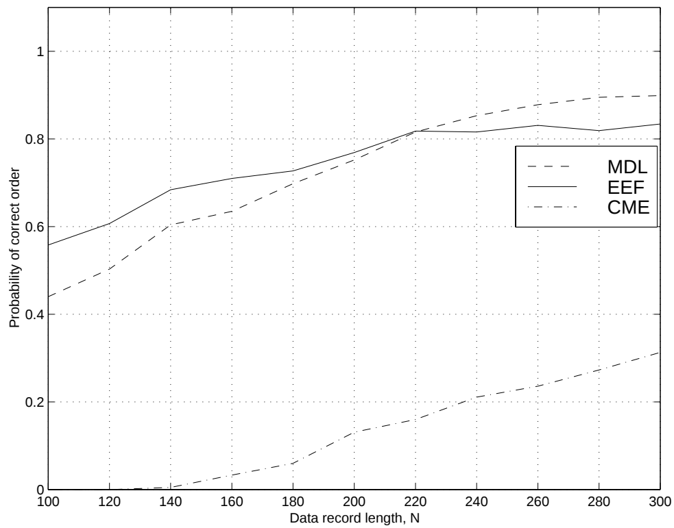
Figure 4: Probability of correct model order for sinusoids versus data record length
