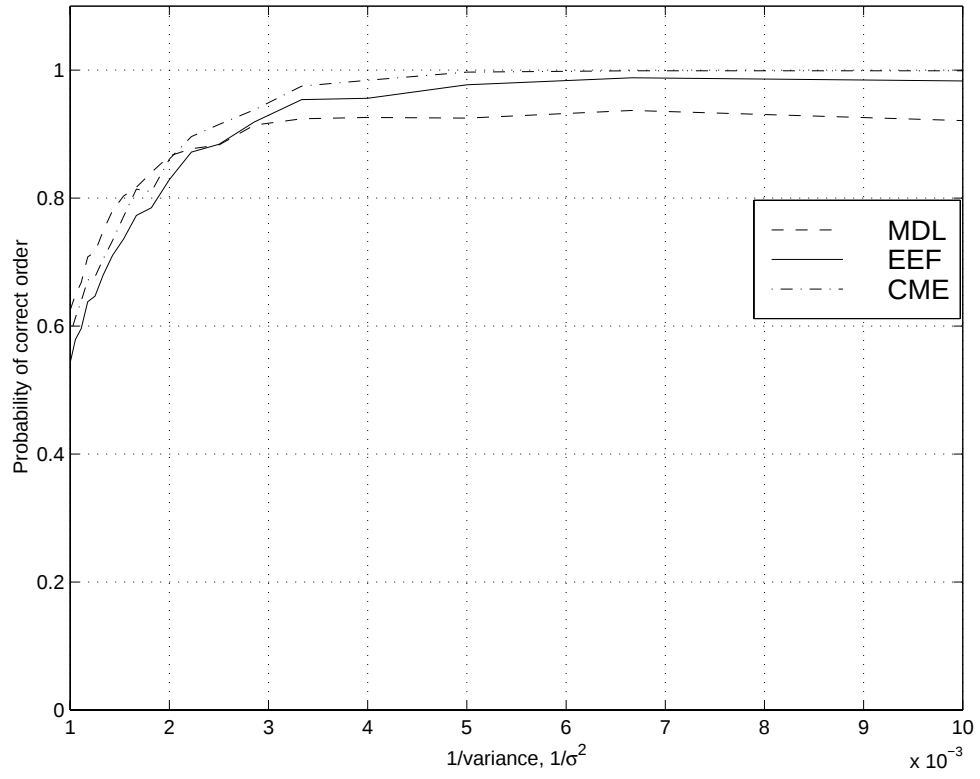
Figure 3: Probability of correct model order for polynomial versus inverse noise variance
