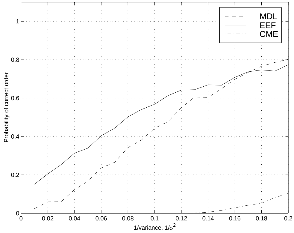
Figure 5: Probability of correct model order for sinusoids versus inverse noise variance
