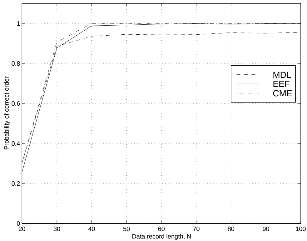
Figure 2: Probability of correct model order for polynomial versus data record length
