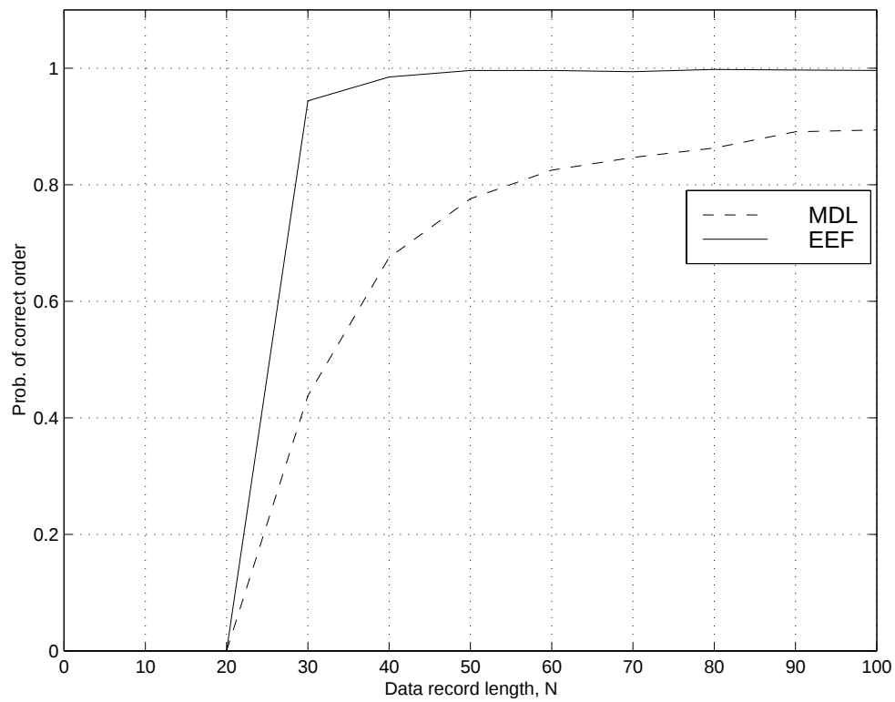
Figure 6: Probability of correct model order for AR process of order 4
